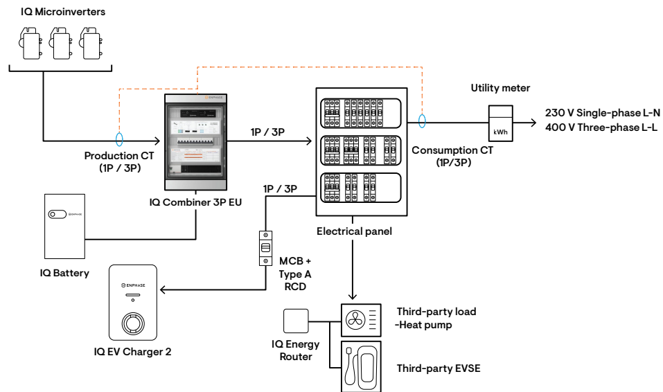
Figure 4: Integrated with an Enphase PV + Battery system + HEMS configuration
